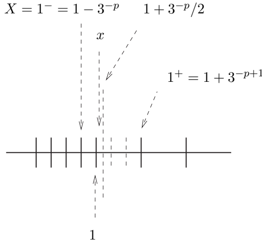
Figure 2.7: This example shows that Property 2 is not true in radix 3. Here, x satisfies 1 < x < 1 + \frac{1}{2}3^{-p} and X = 1^- = 1 - 3^{-p} (if v is a floating-point number, v^- denotes its predecessor, namely, the largest floating-point number less than v , and v^+ denotes its successor). We have \text{HarrisonUlp}(x) = 3^{-p+1} , and |x - X| < 3^{-p+1}/2 , so that |x - X| < \frac{1}{2} \text{HarrisonUlp}(x) . However, X \neq \text{RN}(x) .
