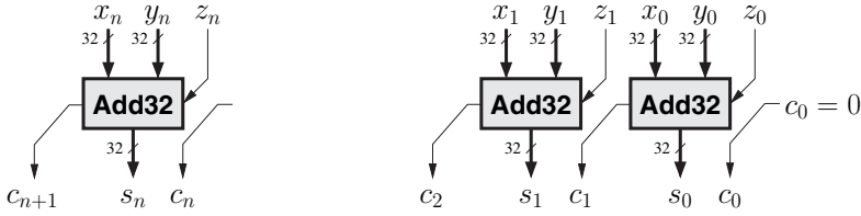
Figure 9.6: Partial carry-save addition.
