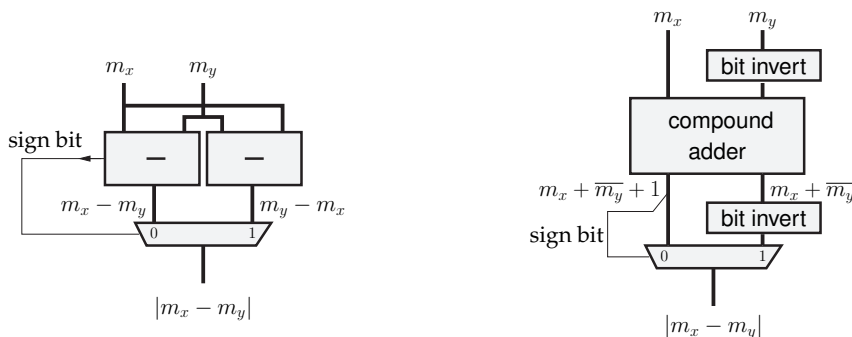
Figure 9.12: Possible implementations of significant subtraction in the close path.
