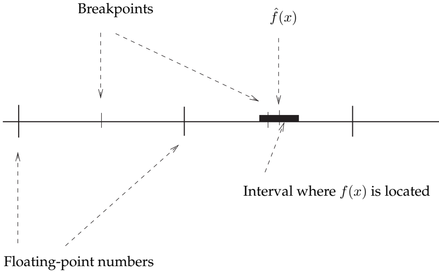
Figure 12.2: In this example (assuming rounding to nearest), the interval around \hat{f}(x) where f(x) is known to be located contains a breakpoint. We do not have enough information to provide a correctly rounded result.
