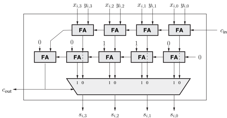
Figure 9.3: An implementation of the decimal DA box.
